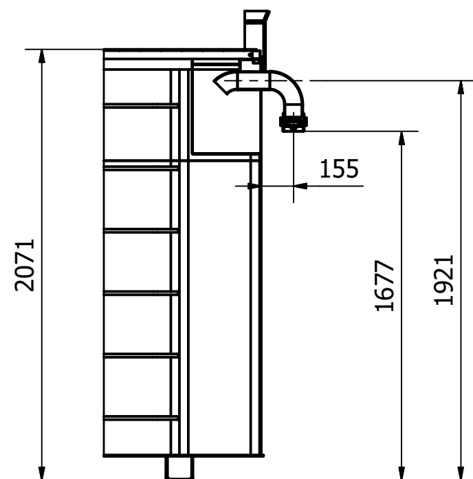
C-C ( 1 :25 )
